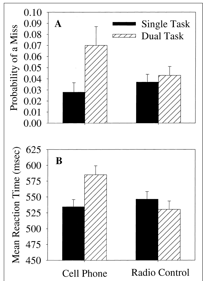
Fig. 1. Probability of missing the simulated traffic signals (a) and mean reaction time to the simulated traffic signals (b) in single- and dual-task conditions in Experiment 1.
